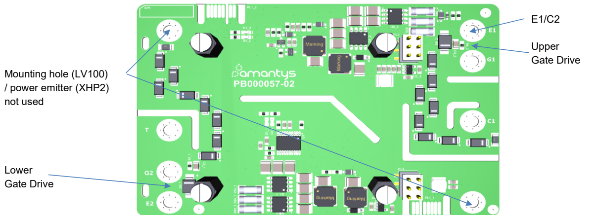
Top View of nHPD2 bottom board showing IGBT connections
